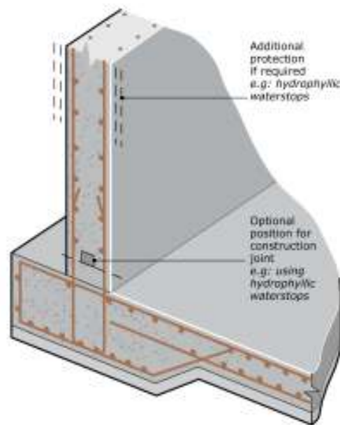
Figure 8: Example of structurally integral protection (Type B) and sketch showing typical detail
