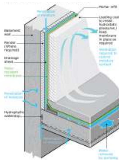
Figure 6: Typical waterproofing requirements for a Grade 3/4 basement
