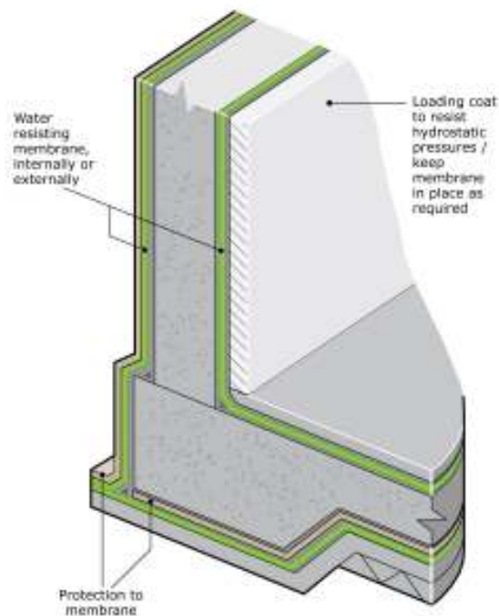
Figure 7: Example of tanked protection (Type A) and sketch showing typical detail.
